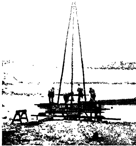
Fig. 14. —Winch Boring in Progress.
